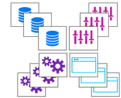
Microservices + APIs
